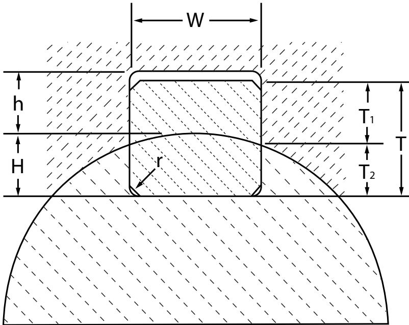
Keyway and Key Size Dimension Reference
